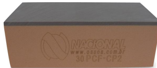
30PCF-CP2 - Block for biomechanical tests 30 pcf with 2 mm cortical W 4,5 X L 9,5 X H 3,2 CM
