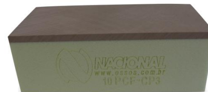
10PCF-CP3 - Block for biomechanical tests 10 pcf with 3 mm cortical W 4,5 X L 9,5 X H 3,3 CM
